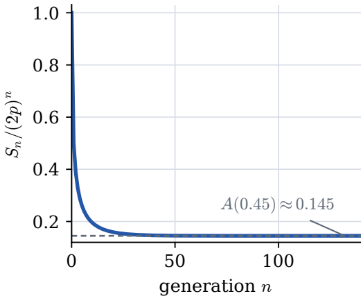
Subcritical: p = 0.45
